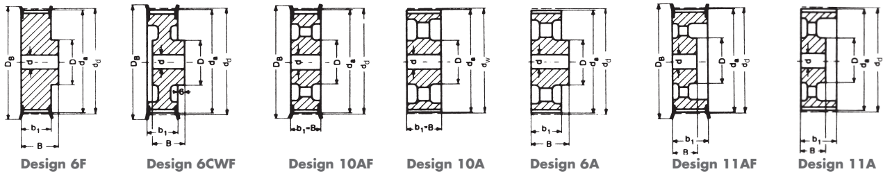
Profile H – Tooth pitch 12.7 mm and width code 150 – belt width 38.1 mm
